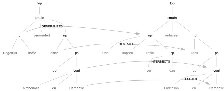
Figure 5.1: Example of two (partially) aligned syntactic trees
