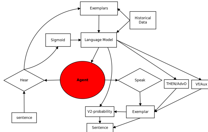
Figure 1: Schematic representation of an agent.
